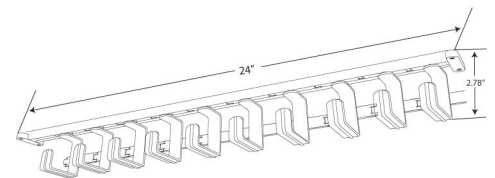
TOP MOUNTED
