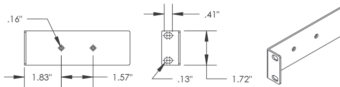
MOUNTING BRACKET (2) INCLUDED
